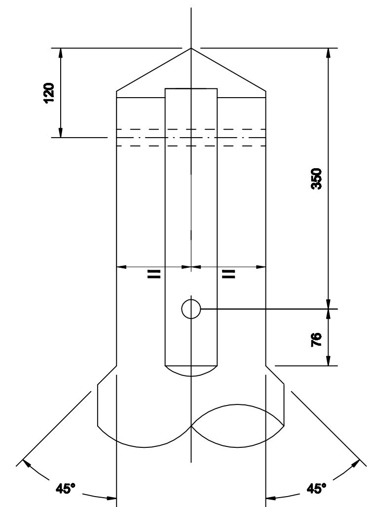
SCALE 1:5
